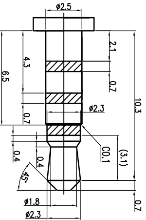
Male Plugs Dimensions
