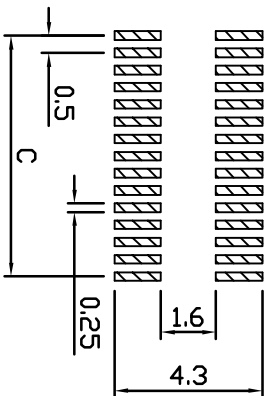
P. C. B LAYOUT
